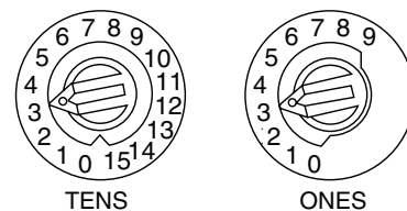
FIGURE 2. ROTARY ADDRESS SWITCHES:
