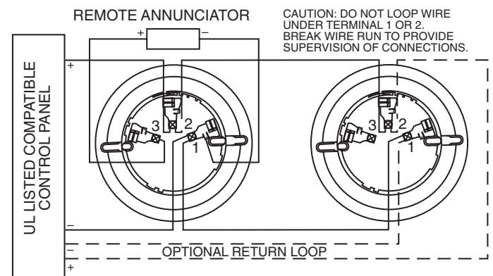
FIGURE 1. WIRING DIAGRAM:
